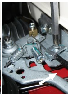
4 ATTACH THE THROTTLE COVER
